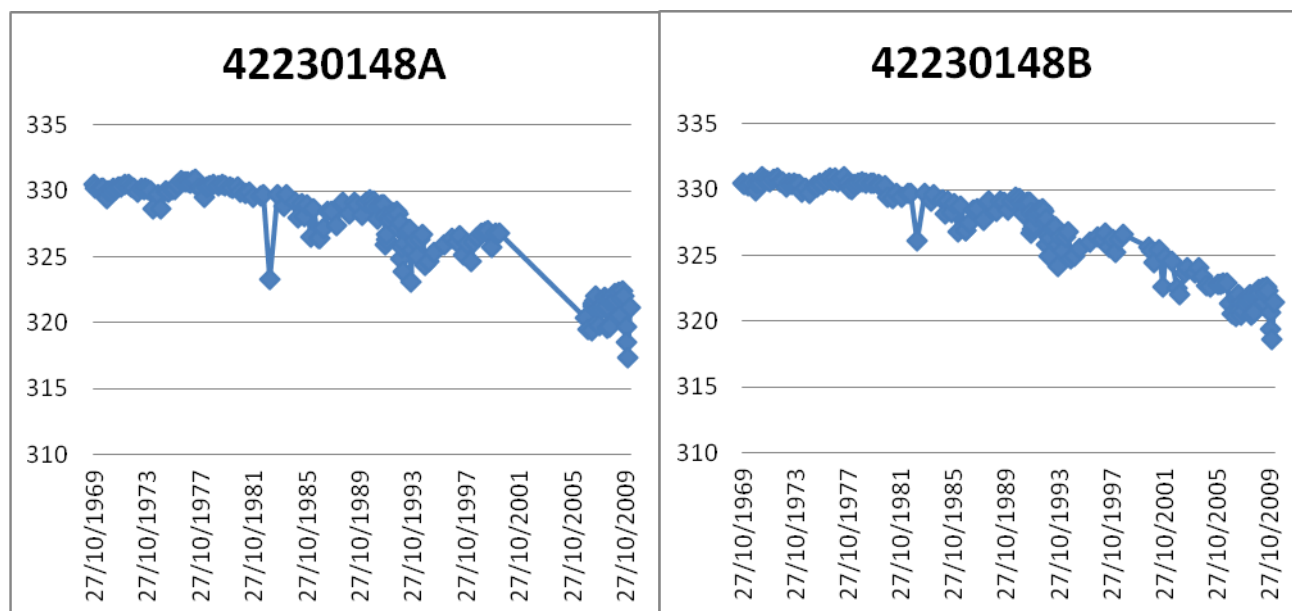
Figure 5 (f) - Bore 42230148 Hydrographs; 42230148A pipe seated at 289.5 m; 42230148B pipe seated at 309.3 m.
